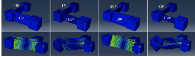
Figure 22: Representative simulations conducted in Abaqus
